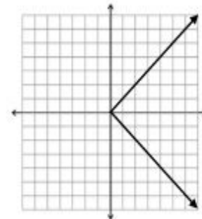
Non-function absolute value: x = |y|
